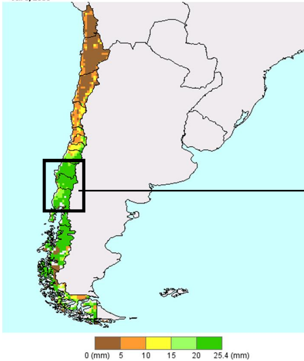
Surface Soil Moisture (SMAP) Jul. 1, 2018
